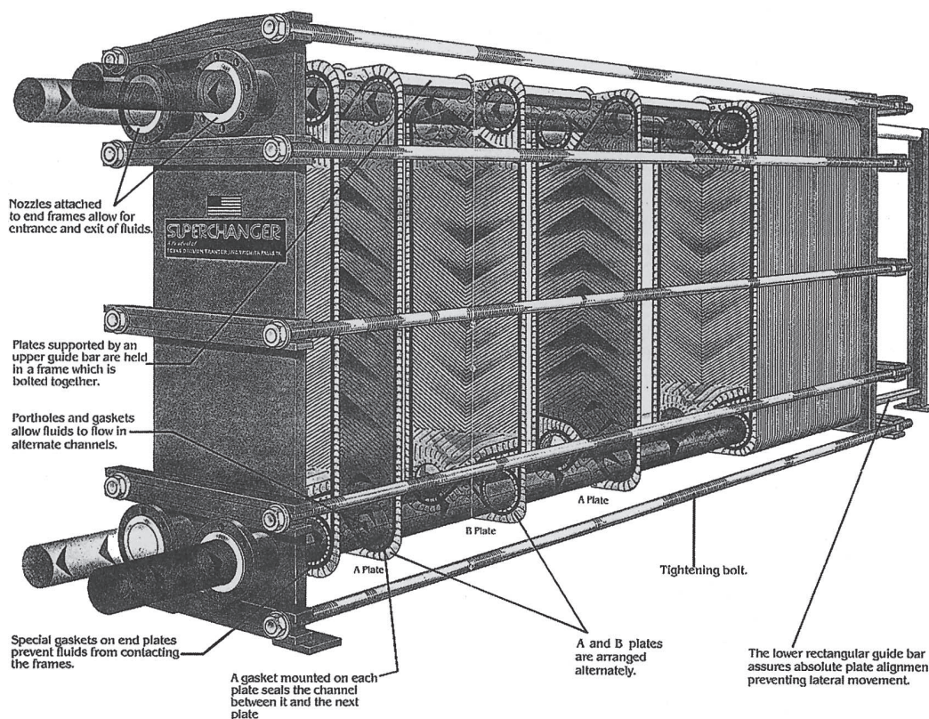
FIGURE 13-6 A plate-and-frame liquid-to-liquid heat exchanger (courtesy of Trane Corp.).
