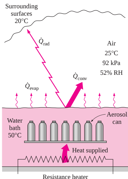
FIGURE 14-54 Schematic for Example 14-13.
