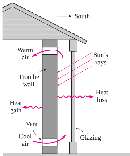
FIGURE 5-46 Schematic of a Trombe wall (Example 5-6).
