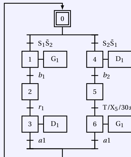
Figure 2.6: Système chariot
